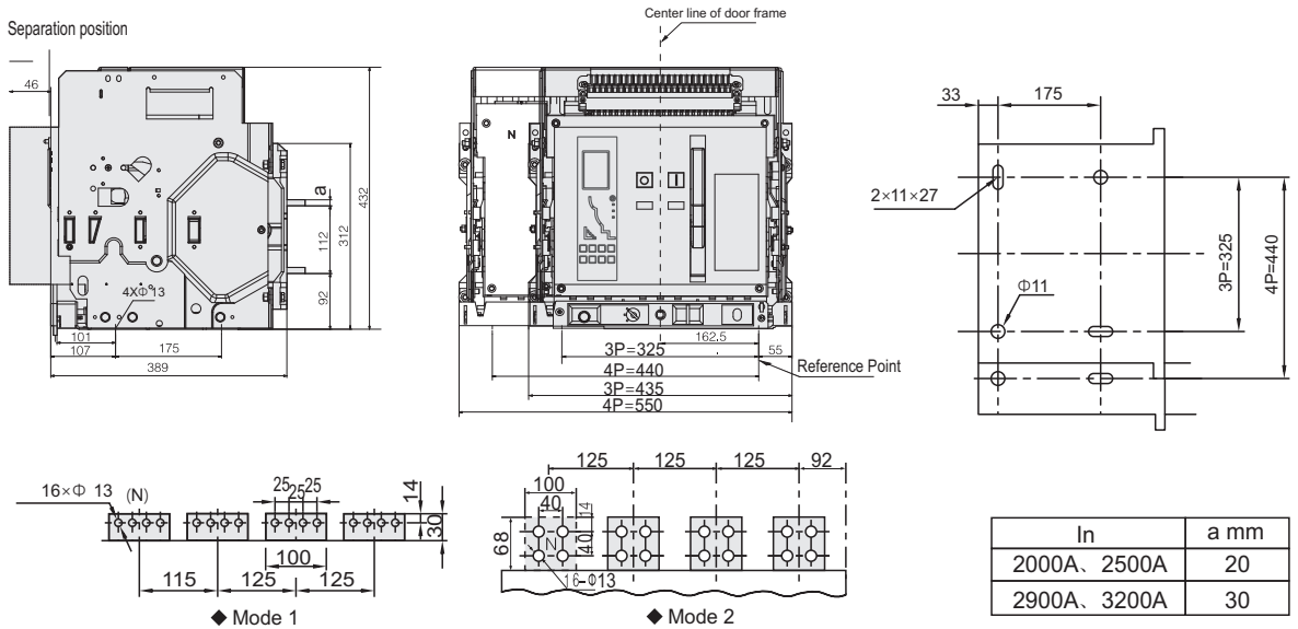
6.12 The shape of YCW3-3200A drawer circuit breaker and installation size are shown in the Figure 26.
